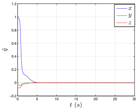
Fig. 2: Observer 1: Attitude Error \tilde{q}
