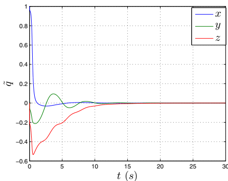
Fig. 3: Observer 2: Attitude Error \tilde{q}
