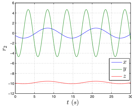
Fig. 1: System Apparent Accel. r_2(t) ( m/s^2 )
